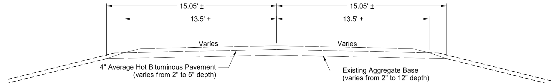
EXISTING TYPICAL SECTION
