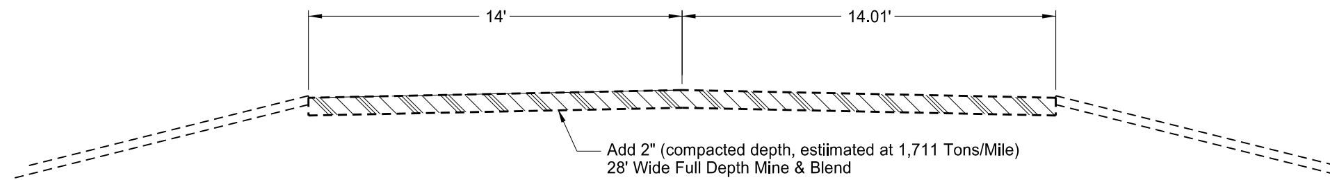
FULL DEPTH RECLAMATION TYPICAL SECTION
