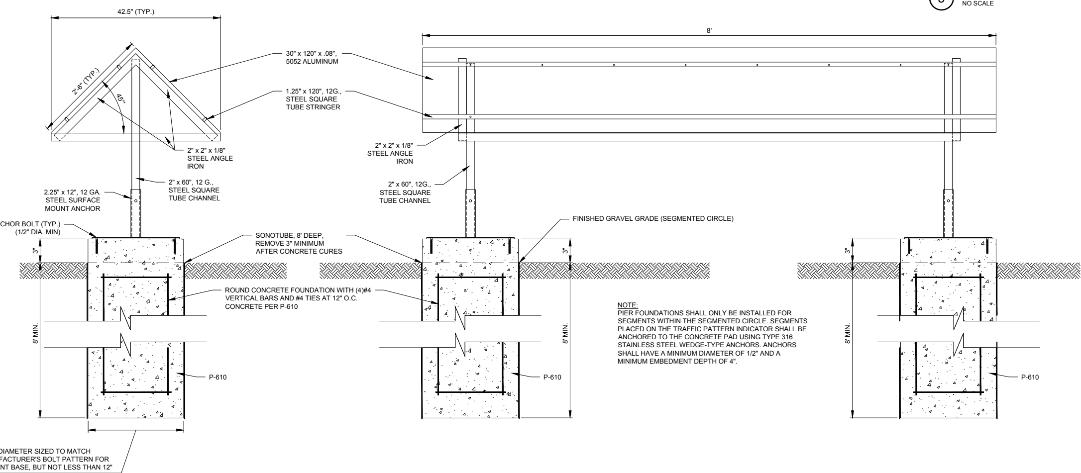
4 SEGMENTED CIRCLE - SEGMENT SIDE VIEW NO SCALE
