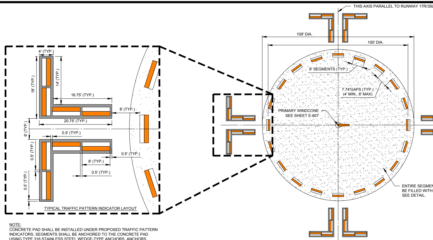
1 SEGMENTED CIRCLE MARKER AND PRIMARY WINDCONE LAYOUT NO SCALE
