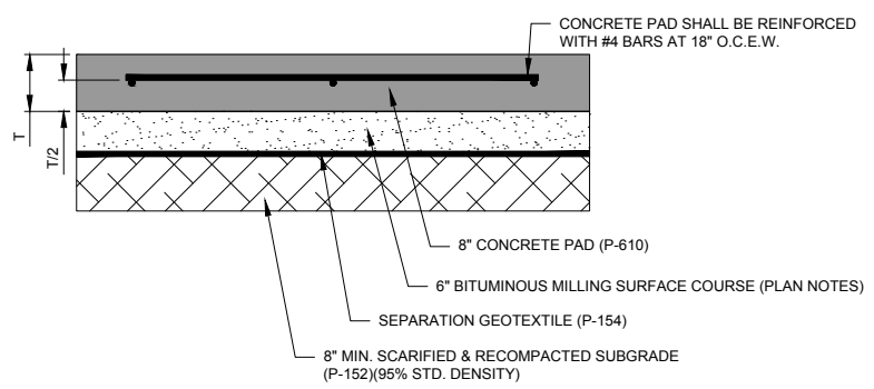
3 TRAFFIC PATTERN INDICATOR CONCRETE PAD SECTION NO SCALE
