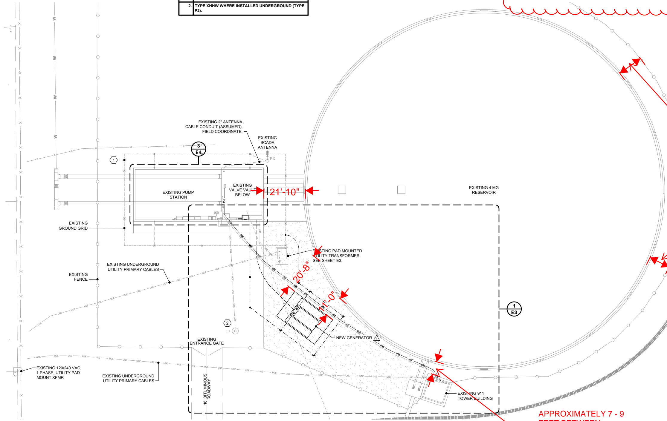
1 SOUTH SIDE PUMP STATION ELECTRICAL SITE PLAN 15' 0 15' 30' NORTH
