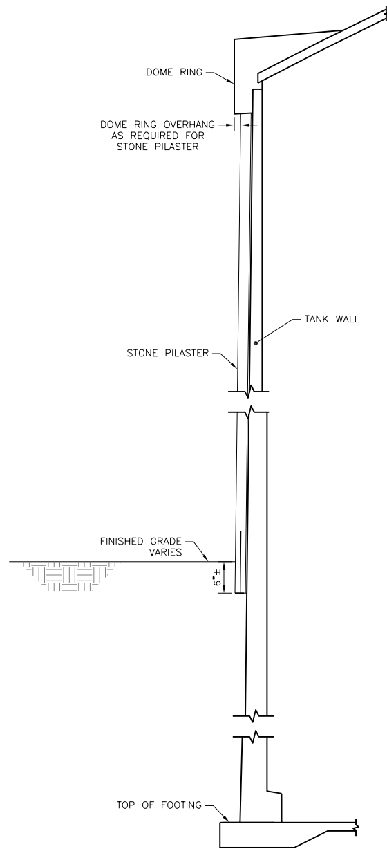
2 P6 RESERVOIR SECTION AT STONE VENEER PILASTER (ALTERNATE BID) SCALE: NONE
