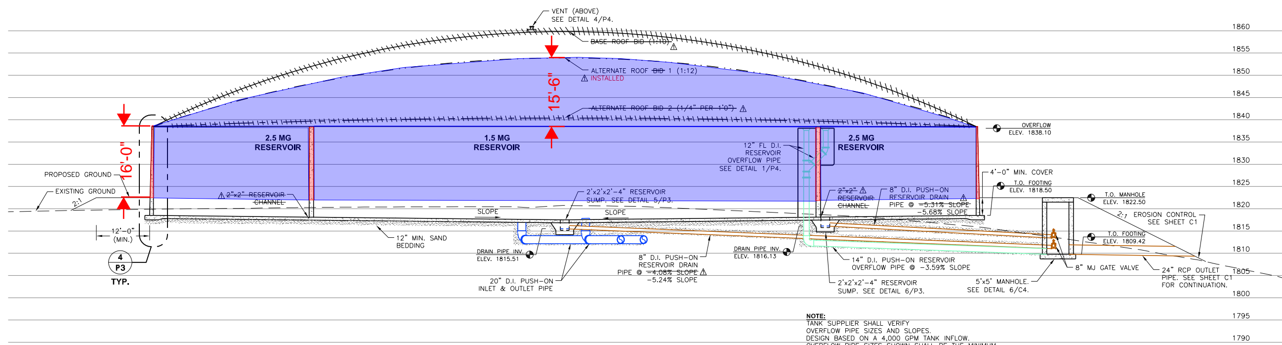
2 P2 PROPOSED IMPROVEMENTS RESERVOIR - CROSS SECTION 8 4 0 4 8 12 16
