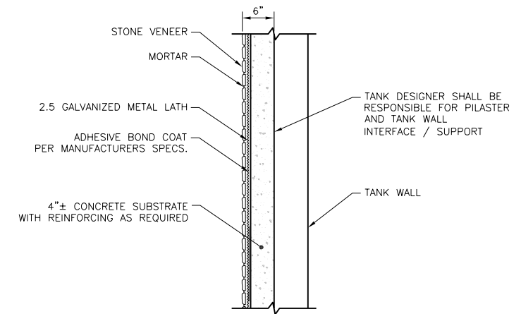
3 P6 STONE PILASTER CONCRETE SUBSTRATE WITH STONE VENEER DETAIL SCALE: NONE
