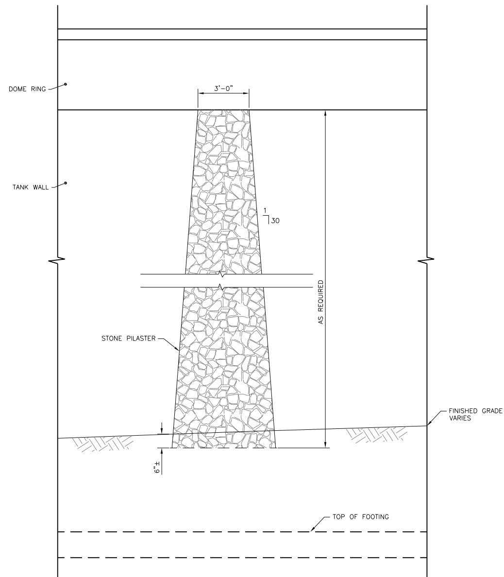
1 P6 RESERVOIR ELEVATION AT STONE VENEER PILASTER (ALTERNATE BID) SCALE: NONE
