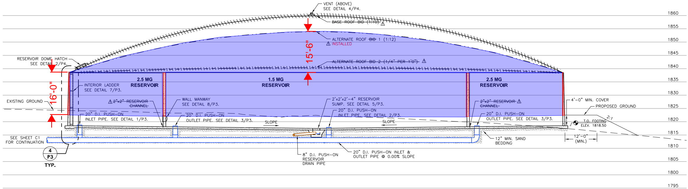
1 P2 PROPOSED IMPROVEMENTS RESERVOIR - CROSS SECTION 8 4 0 4 8 12 16
