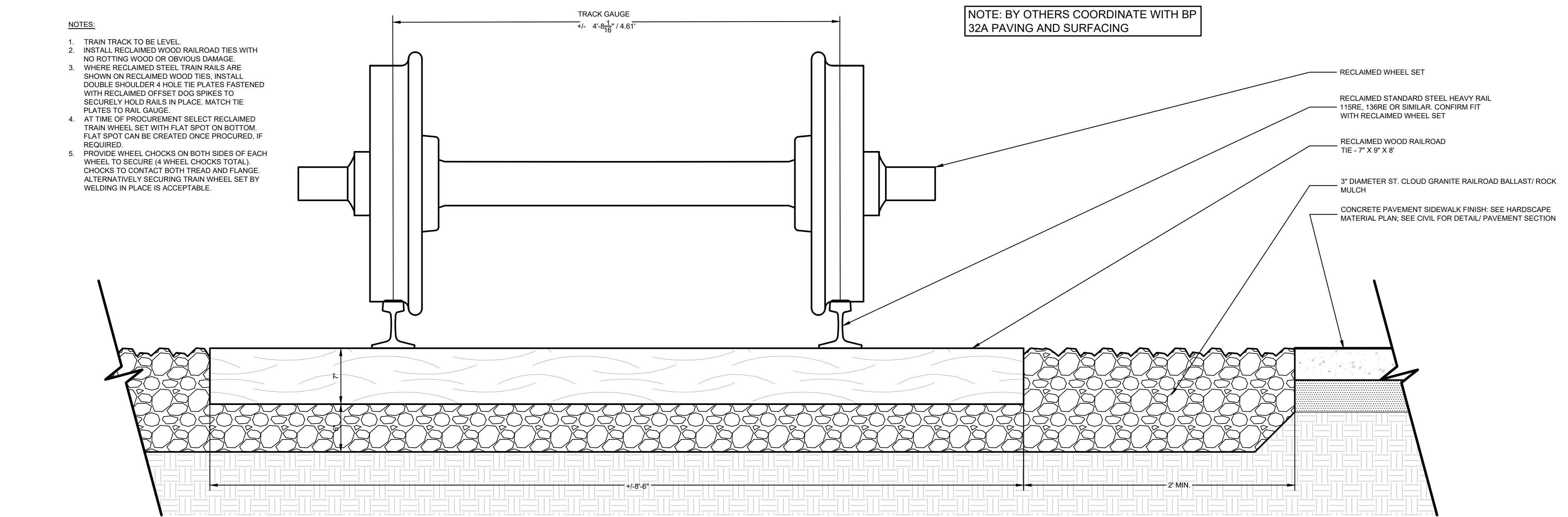
6 TRAIN WHEELS & AXLE DETAIL SCALE: 1 1/2" = 1'-0"
